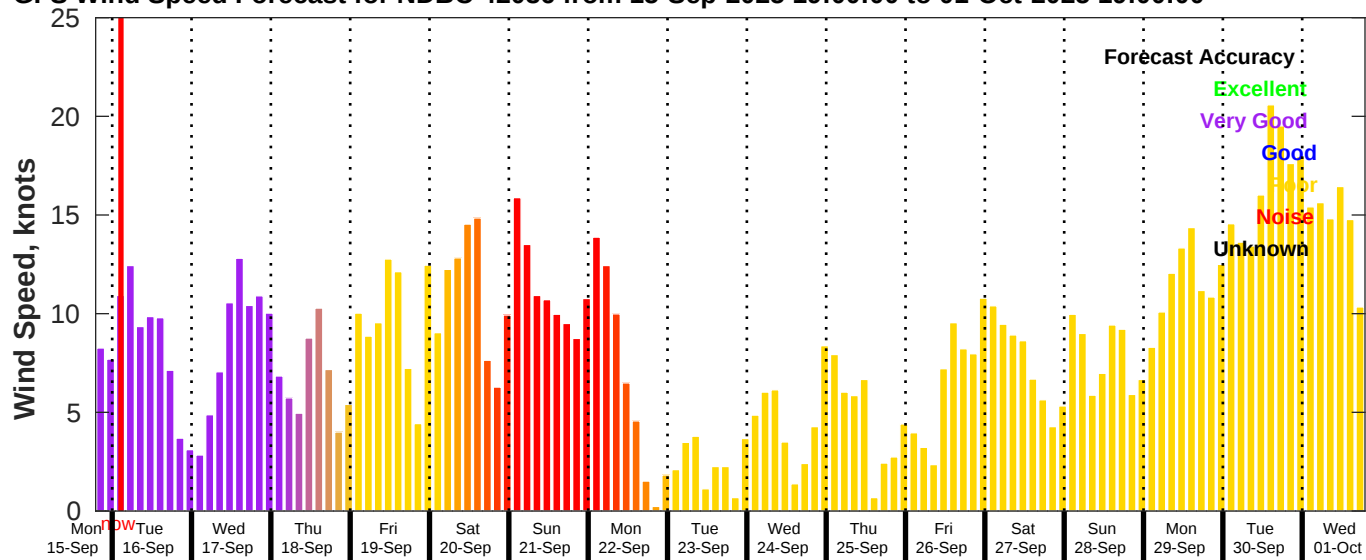
GFS Wind Speed Forecast for NDBC 42036 from 15-Sep-2025 19:00:00 to 01-Oct-2025 19:00:00
