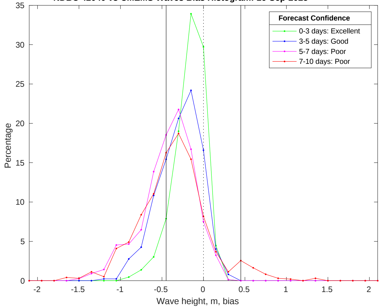
NDBC 42040 vs CMEMS Waves Bias Histogram: 16-Sep-2025
