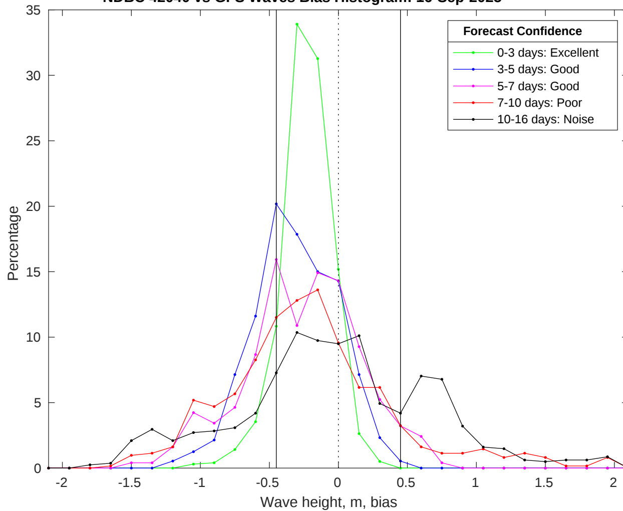
NDBC 42040 vs GFS Waves Bias Histogram: 16-Sep-2025
