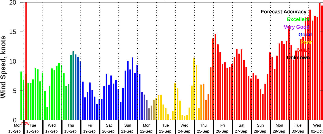
GFS Wind Speed Forecast for NDBC 42040 from 15-Sep-2025 19:00:00 to 01-Oct-2025 19:00:00
