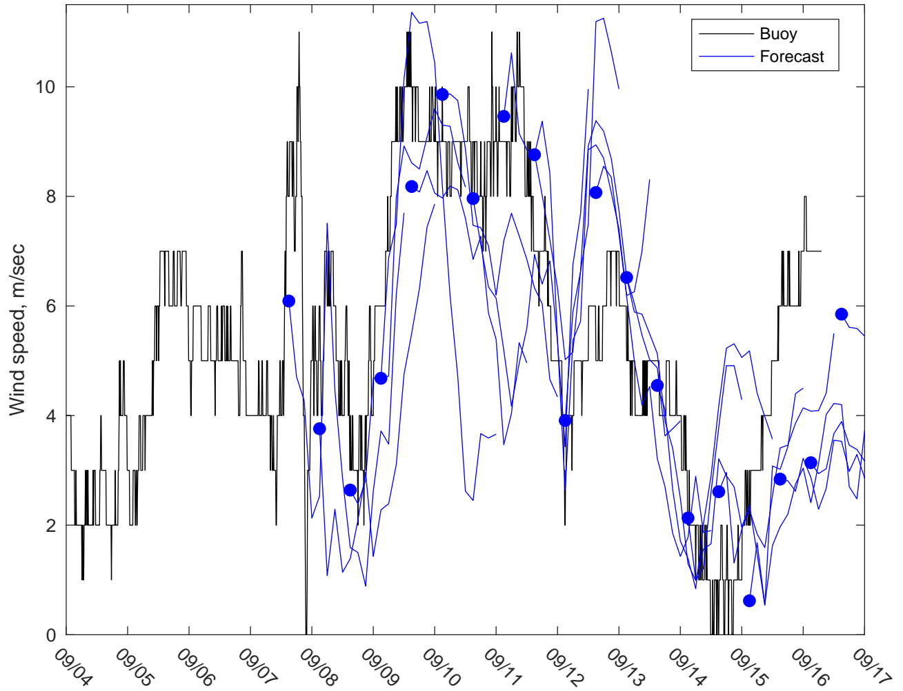
NDBC 44008 vs GFS Winds: 3 to 5 day forecast
