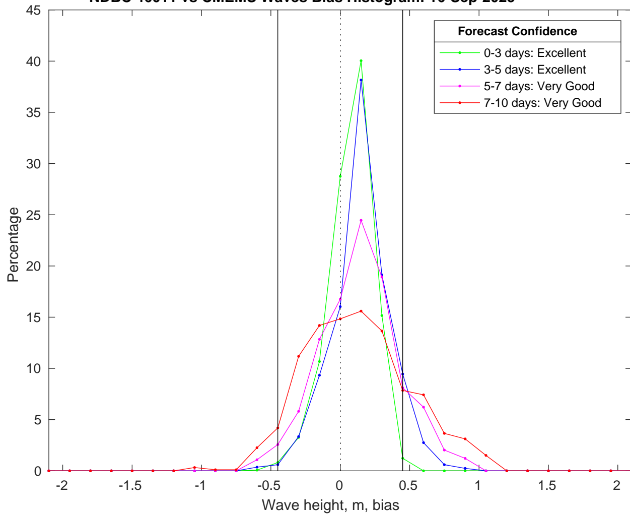
NDBC 46011 vs CMEMS Waves Bias Histogram: 16-Sep-2025
