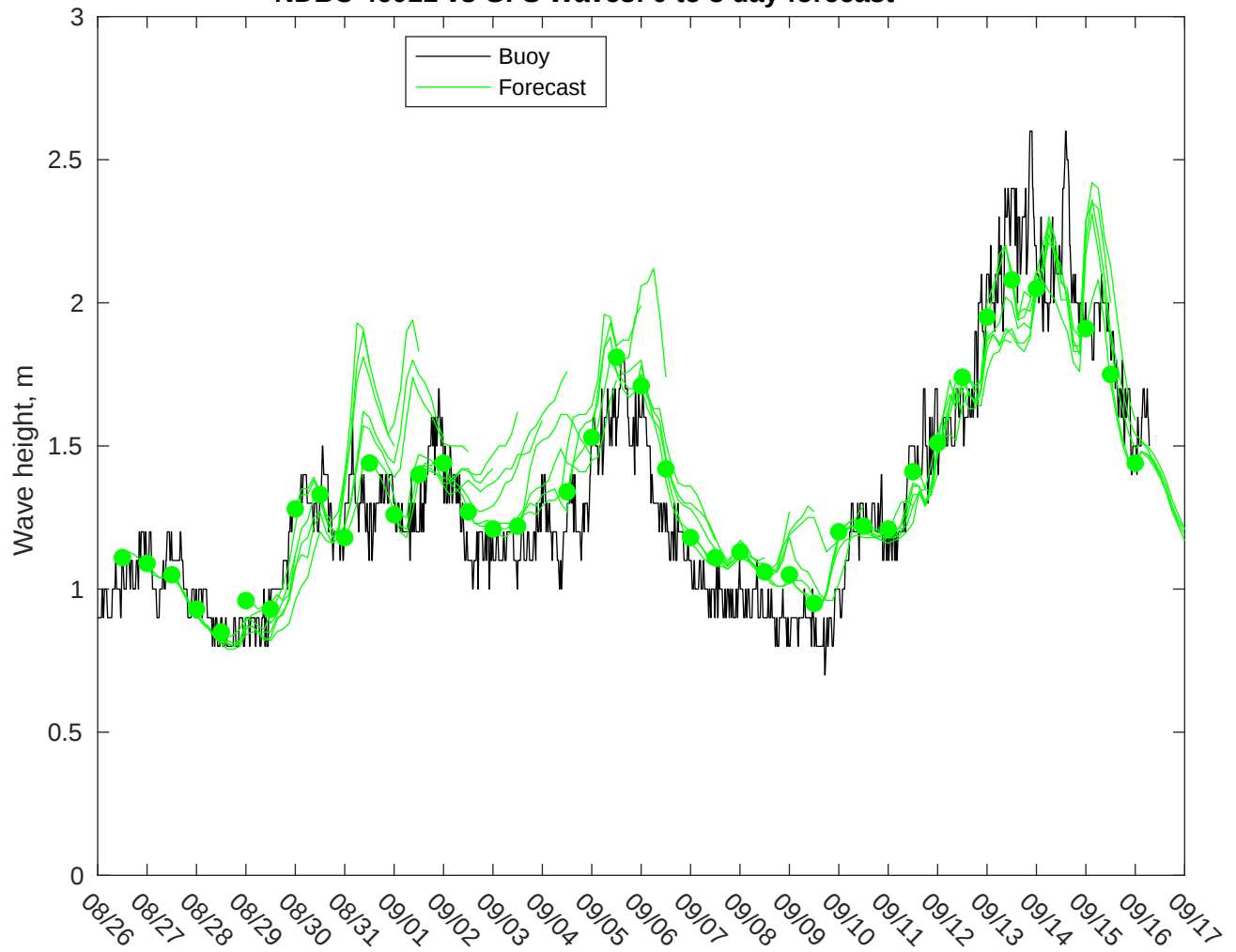
NDBC 46011 vs GFS Waves: 0 to 3 day forecast
