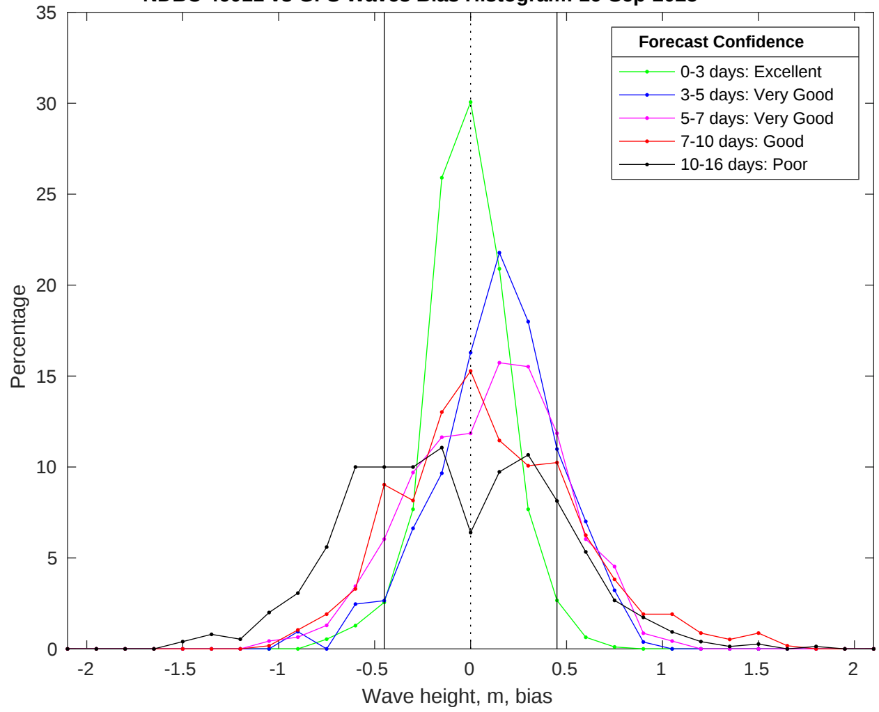
NDBC 46011 vs GFS Waves Bias Histogram: 16-Sep-2025
