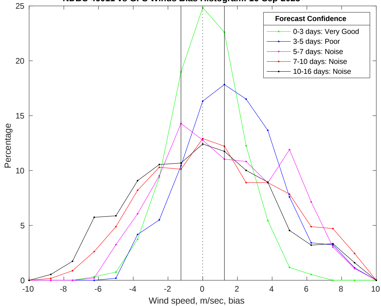
NDBC 46011 vs GFS Winds Bias Histogram: 16-Sep-2025
