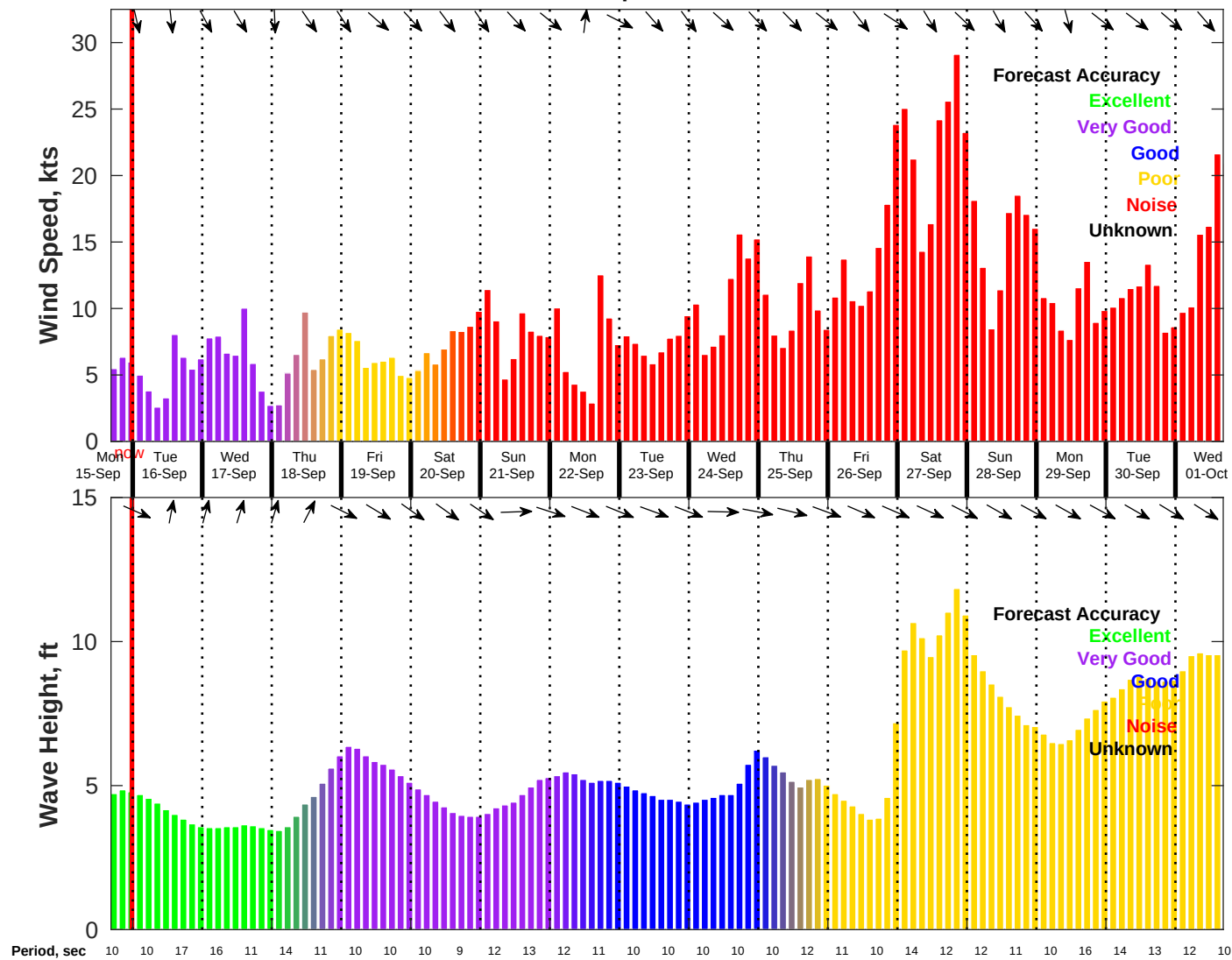
Wind & Wave Forecast for NDBC 46011 from 15-Sep-2025 16:00:00 to 01-Oct-2025 16:00:00
