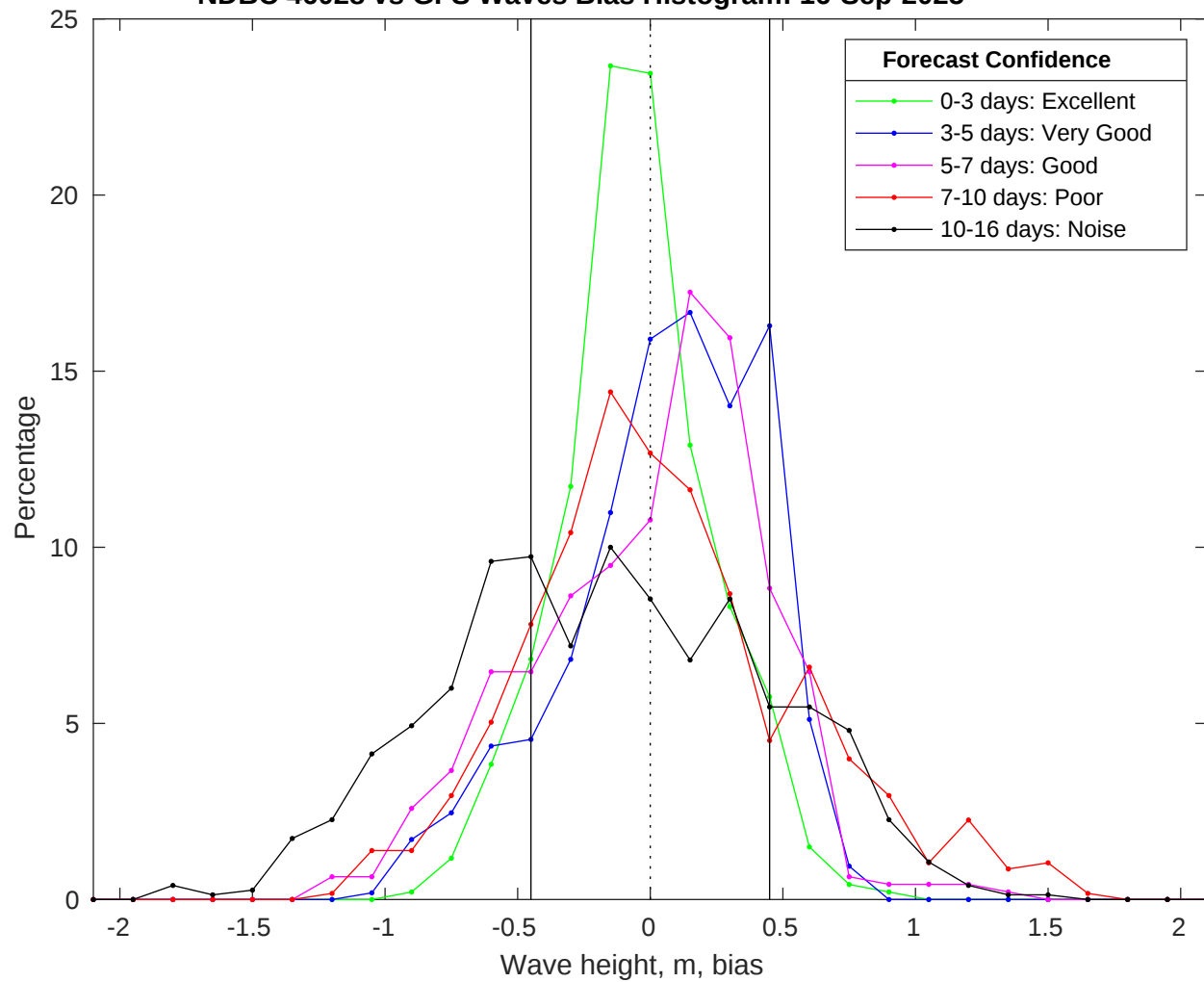
NDBC 46028 vs GFS Waves Bias Histogram: 16-Sep-2025
