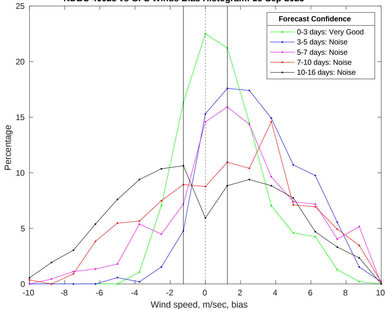
NDBC 46028 vs GFS Winds Bias Histogram: 16-Sep-2025
