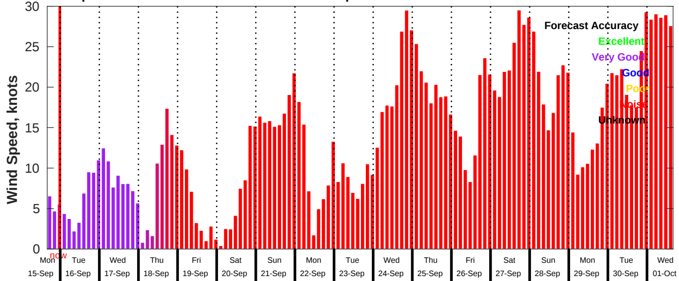
GFS Wind Speed Forecast for NDBC 46028 from 15-Sep-2025 16:00:00 to 01-Oct-2025 16:00:00
