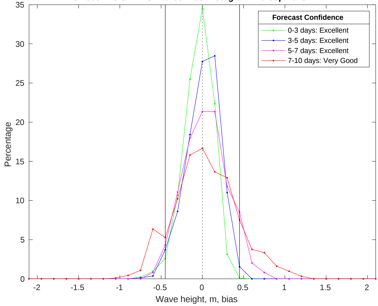
NDBC 46054 vs CMEMS Waves Bias Histogram: 16-Sep-2025
