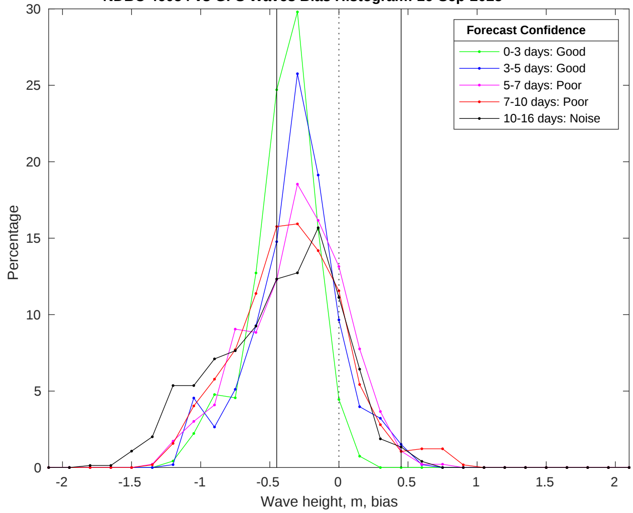
NDBC 46054 vs GFS Waves Bias Histogram: 16-Sep-2025
