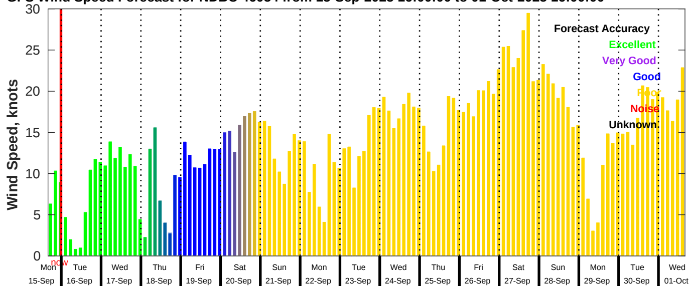
GFS Wind Speed Forecast for NDBC 46054 from 15-Sep-2025 16:00:00 to 01-Oct-2025 16:00:00
