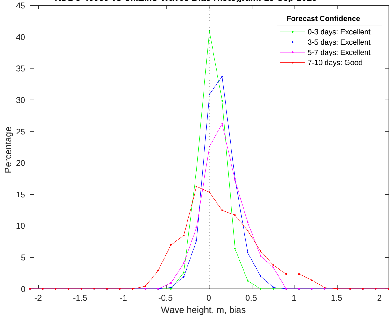
NDBC 46069 vs CMEMS Waves Bias Histogram: 16-Sep-2025
