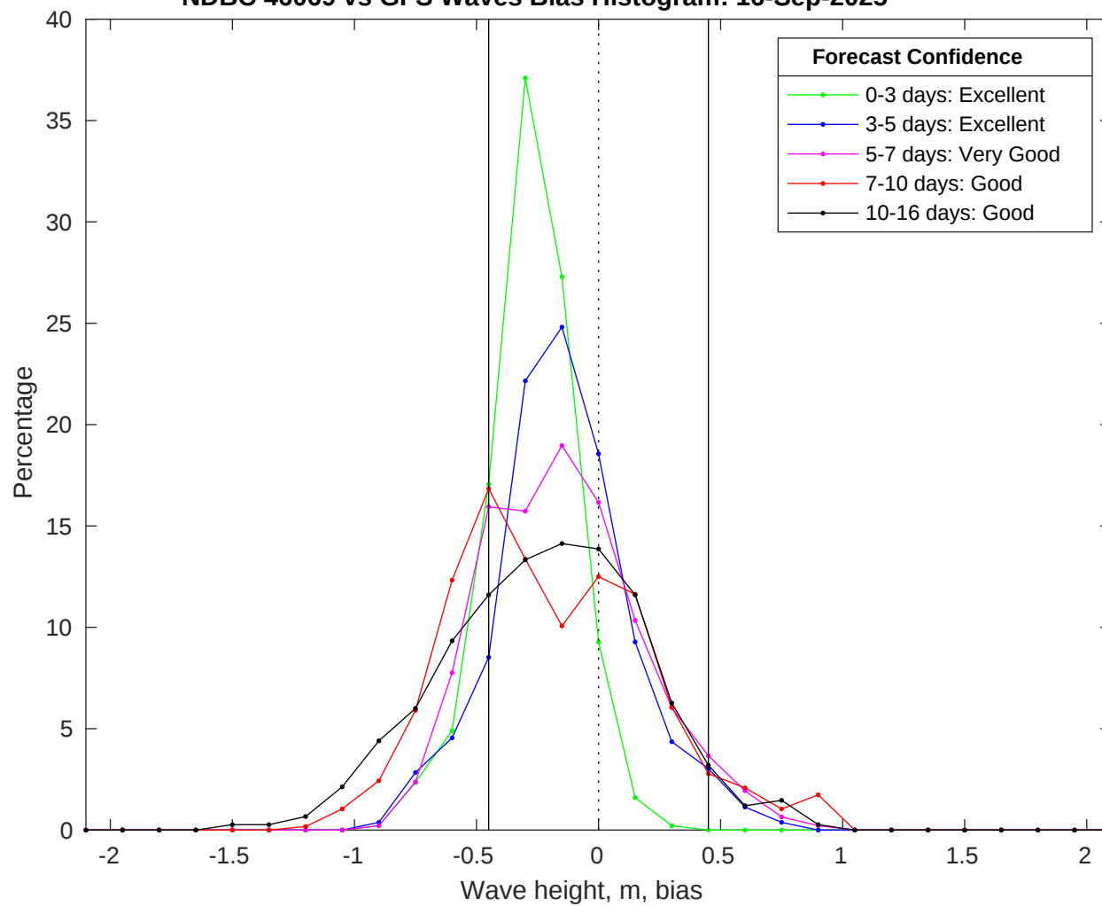
NDBC 46069 vs GFS Waves Bias Histogram: 16-Sep-2025
