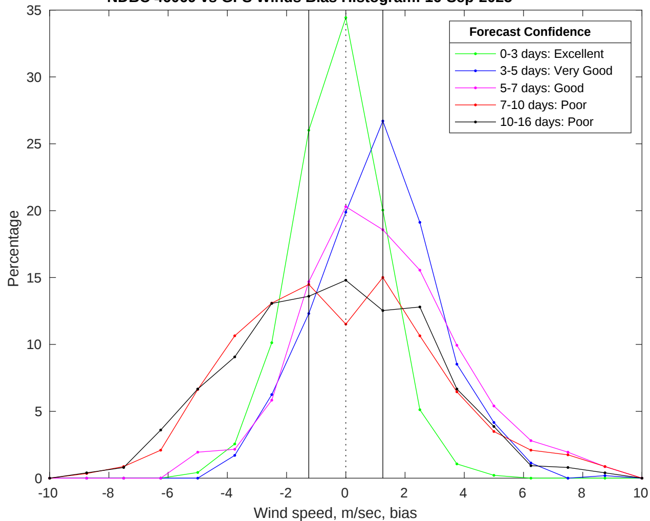
NDBC 46069 vs GFS Winds Bias Histogram: 16-Sep-2025
