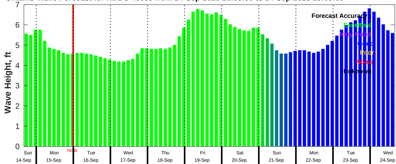
CMEMS Wave Forecast for NDBC 46069 from 14-Sep-2025 16:00:00 to 24-Sep-2025 16:00:00
