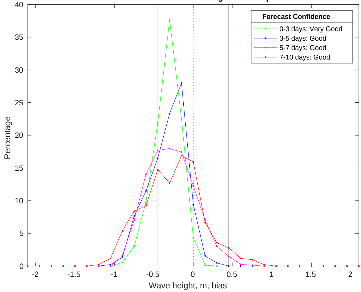
NDBC 51209 vs CMEMS Waves Bias Histogram: 16-Sep-2025
