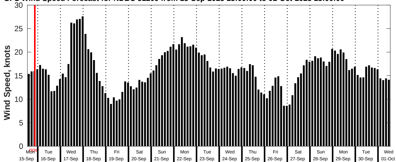
GFS Wind Speed Forecast for NDBC 51209 from 15-Sep-2025 13:00:00 to 01-Oct-2025 13:00:00
