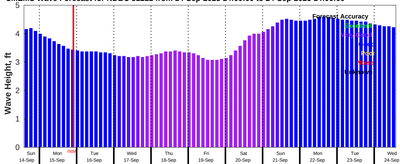
CMEMS Wave Forecast for NDBC 51211 from 14-Sep-2025 14:00:00 to 24-Sep-2025 14:00:00
