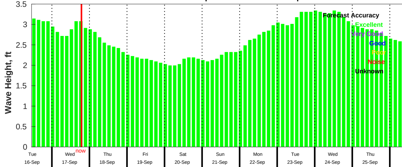
CMEMS Wave Forecast for NDBC 52211 from 15-Sep-2025 11:00:00 to 25-Sep-2025 11:00:00
