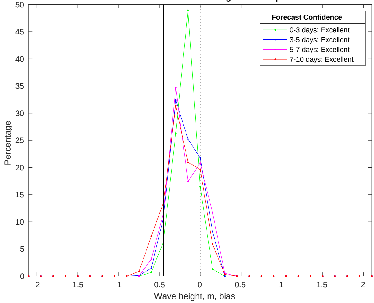
NDBC 52213 vs CMEMS Waves Bias Histogram: 16-Sep-2025
