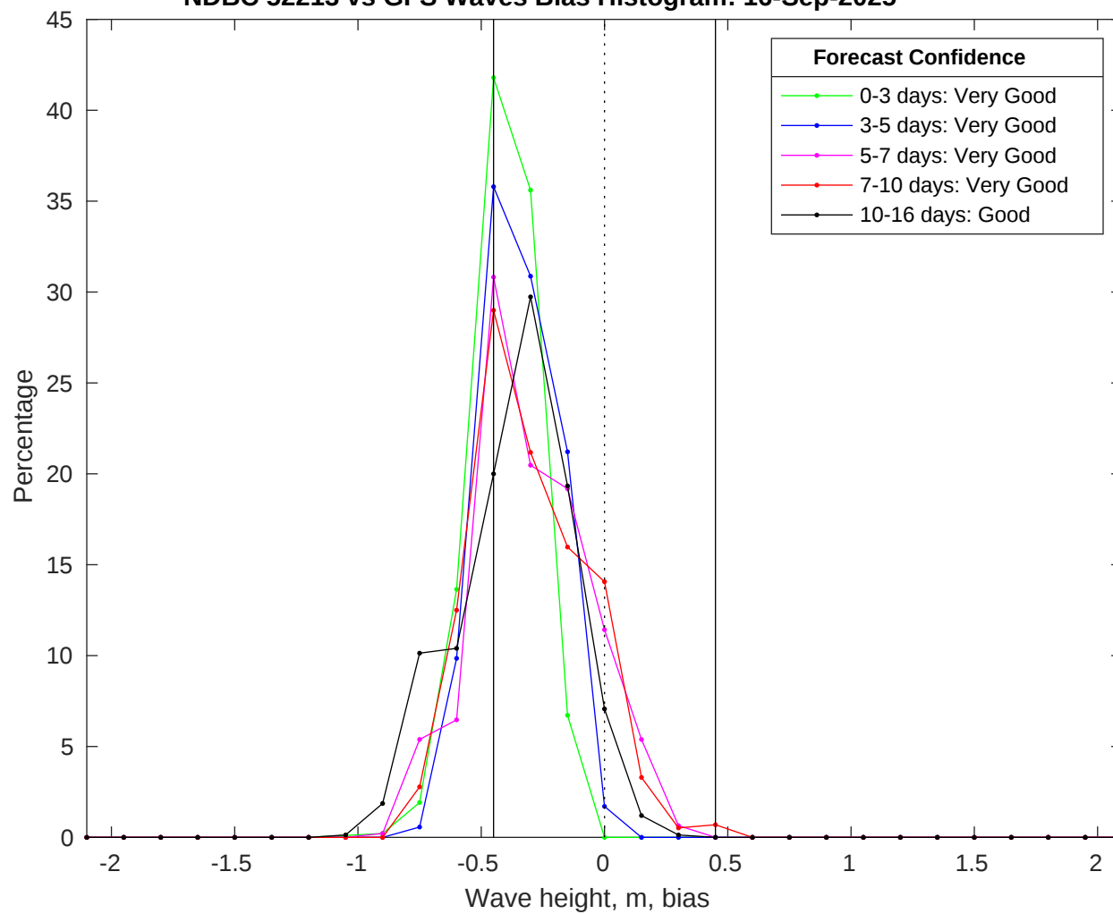
NDBC 52213 vs GFS Waves Bias Histogram: 16-Sep-2025
