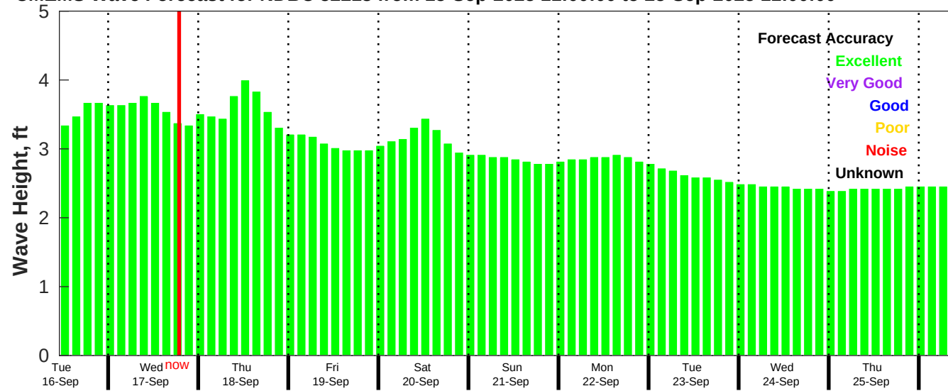
CMEMS Wave Forecast for NDBC 52213 from 15-Sep-2025 11:00:00 to 25-Sep-2025 11:00:00
