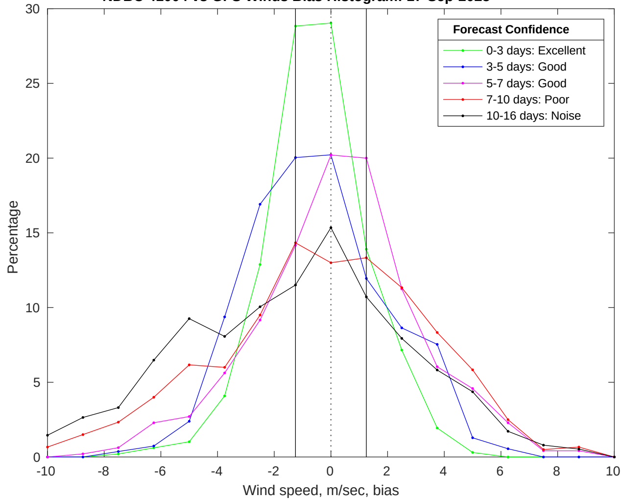
NDBC 41004 vs GFS Winds Bias Histogram: 17-Sep-2025
