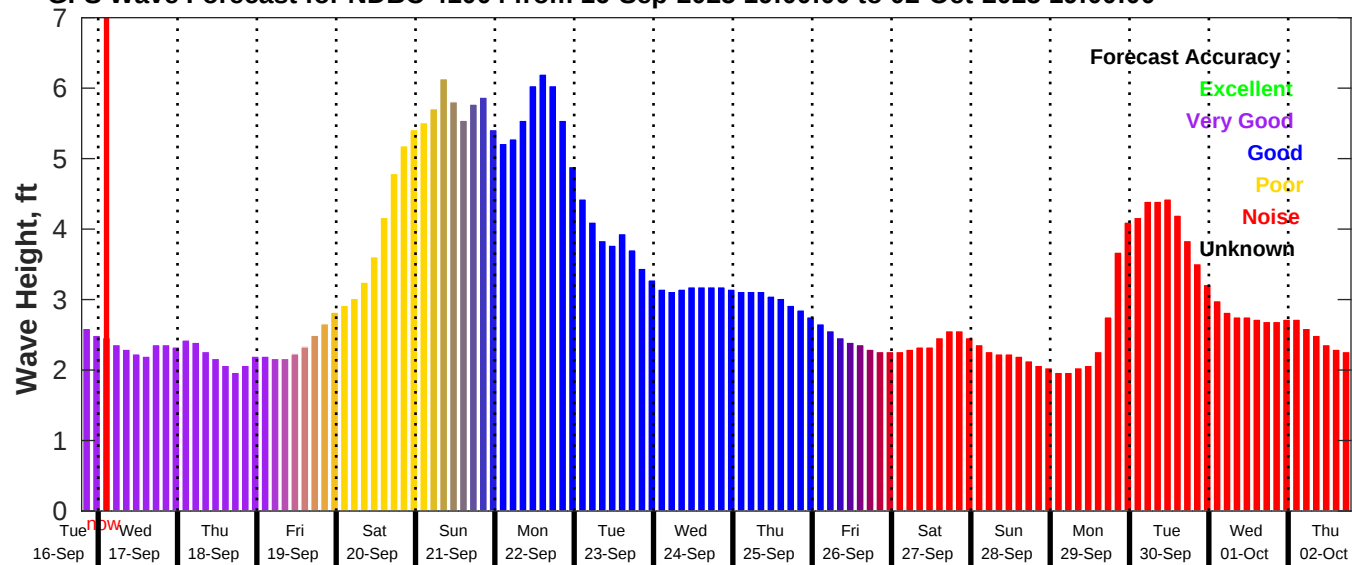
GFS Wave Forecast for NDBC 41004 from 16-Sep-2025 19:00:00 to 02-Oct-2025 19:00:00
