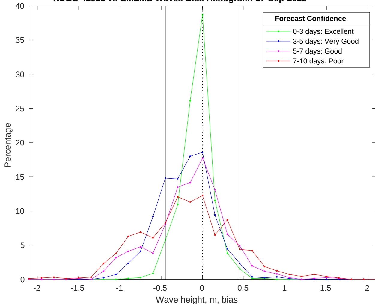
NDBC 41013 vs CMEMS Waves Bias Histogram: 17-Sep-2025
