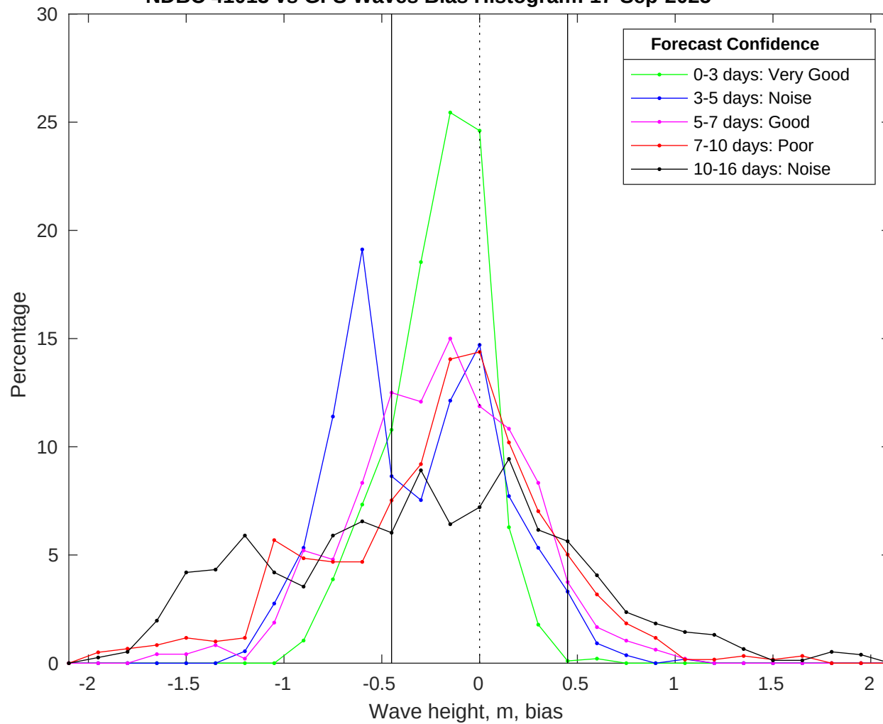
NDBC 41013 vs GFS Waves Bias Histogram: 17-Sep-2025
