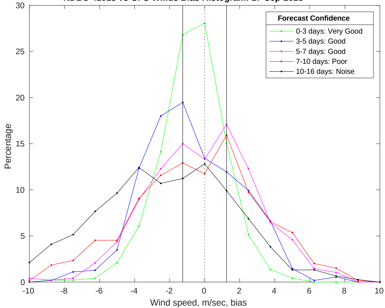
NDBC 41013 vs GFS Winds Bias Histogram: 17-Sep-2025
