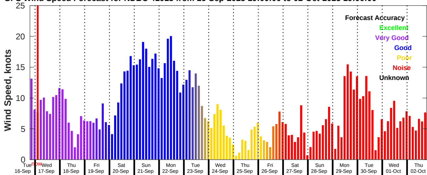
GFS Wind Speed Forecast for NDBC 41013 from 16-Sep-2025 19:00:00 to 02-Oct-2025 19:00:00
