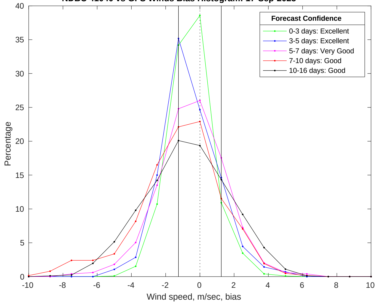
NDBC 41040 vs GFS Winds Bias Histogram: 17-Sep-2025
