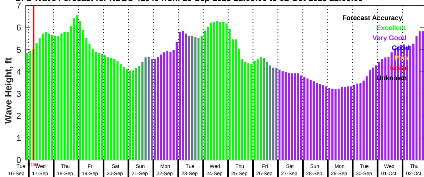
GFS Wave Forecast for NDBC 41040 from 16-Sep-2025 21:00:00 to 02-Oct-2025 21:00:00
