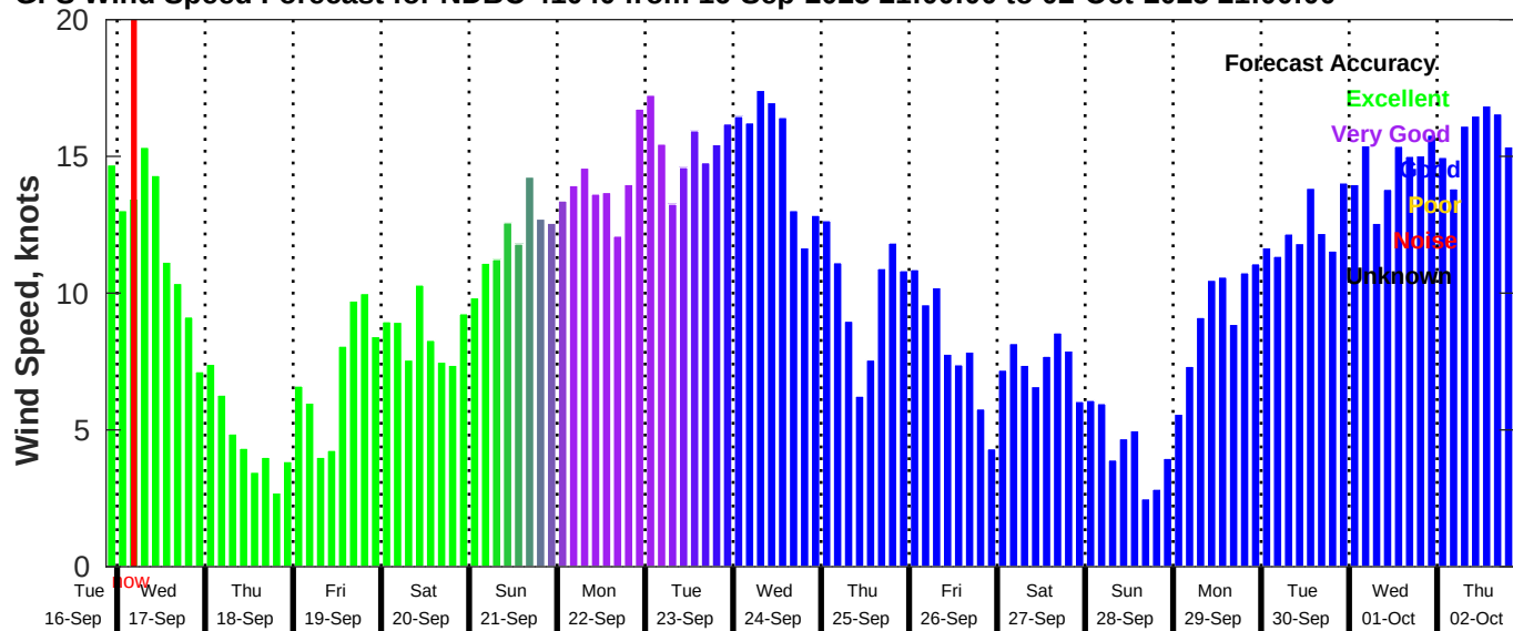
GFS Wind Speed Forecast for NDBC 41040 from 16-Sep-2025 21:00:00 to 02-Oct-2025 21:00:00
