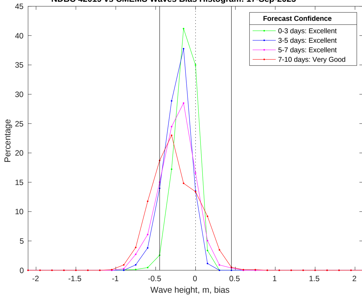
NDBC 42019 vs CMEMS Waves Bias Histogram: 17-Sep-2025
