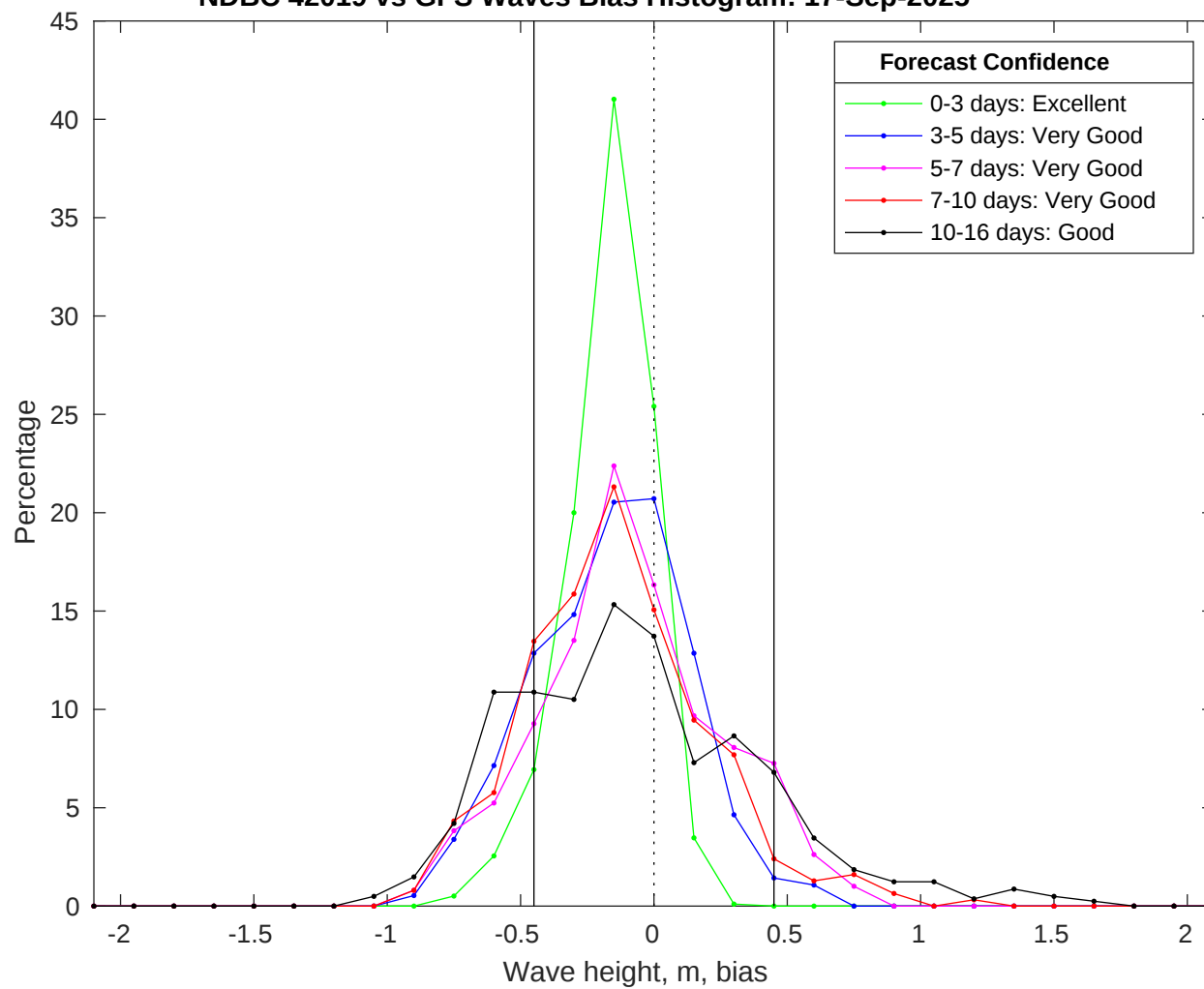
NDBC 42019 vs GFS Waves Bias Histogram: 17-Sep-2025
