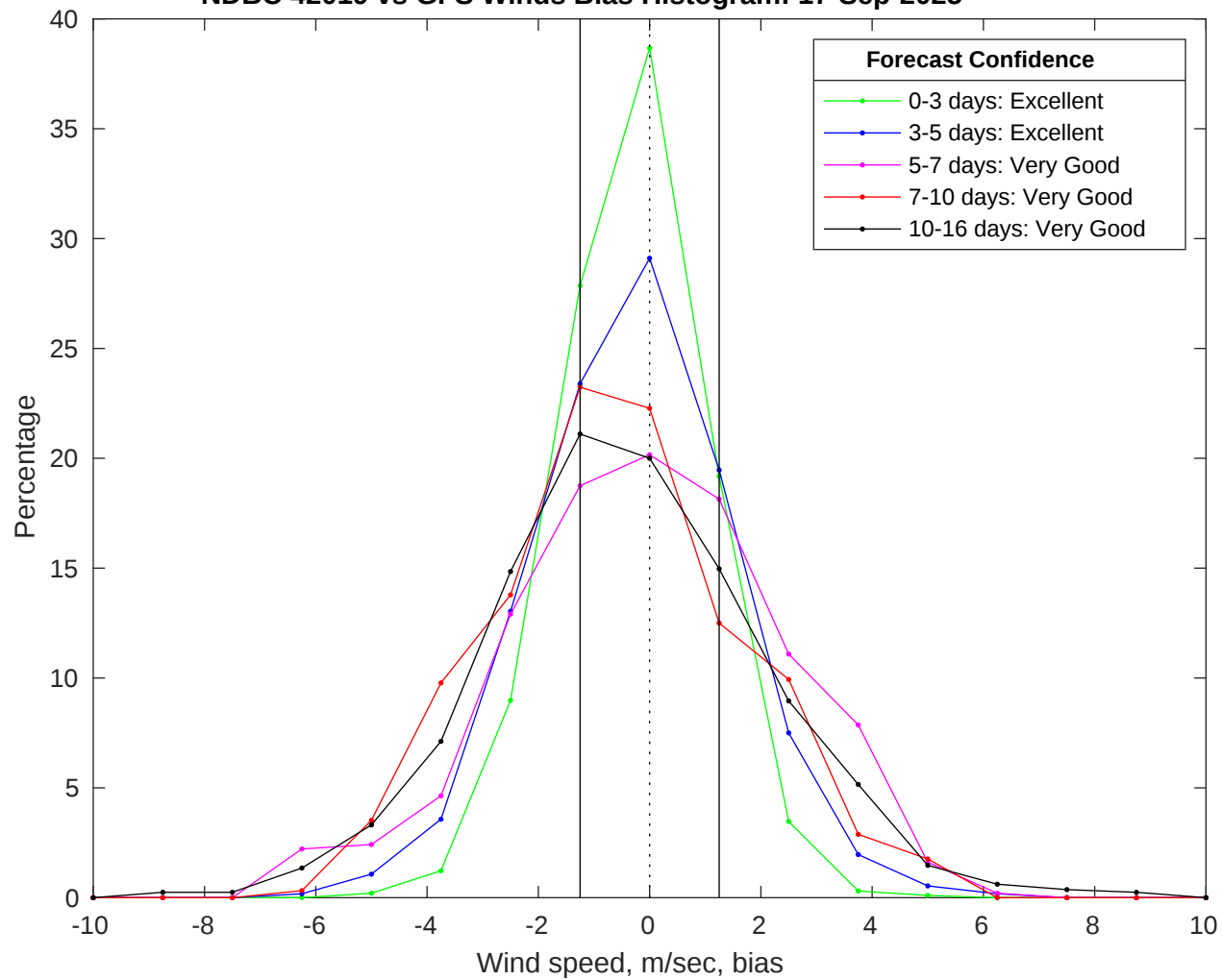
NDBC 42019 vs GFS Winds Bias Histogram: 17-Sep-2025
