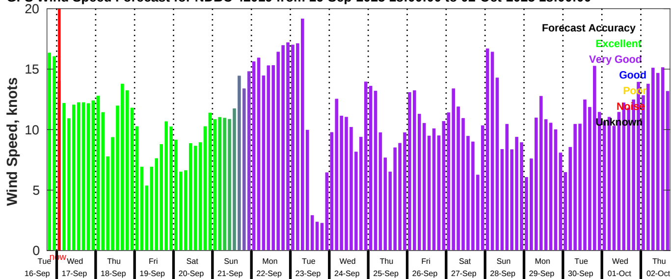
GFS Wind Speed Forecast for NDBC 42019 from 16-Sep-2025 18:00:00 to 02-Oct-2025 18:00:00
