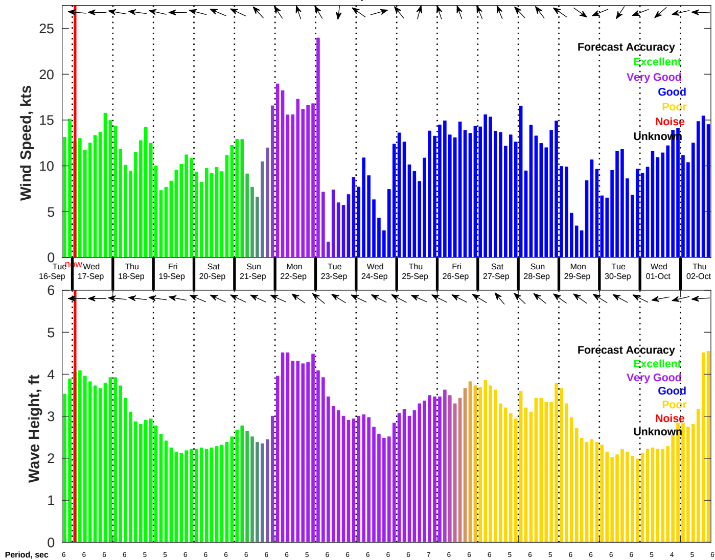
Wind & Wave Forecast for NDBC 42020 from 16-Sep-2025 18:00:00 to 02-Oct-2025 18:00:00
