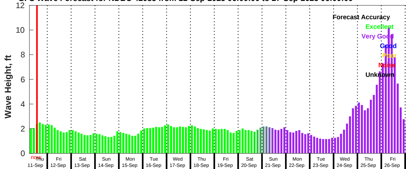
GFS Wave Forecast for NDBC 42035 from 11-Sep-2025 06:00:00 to 27-Sep-2025 06:00:00
