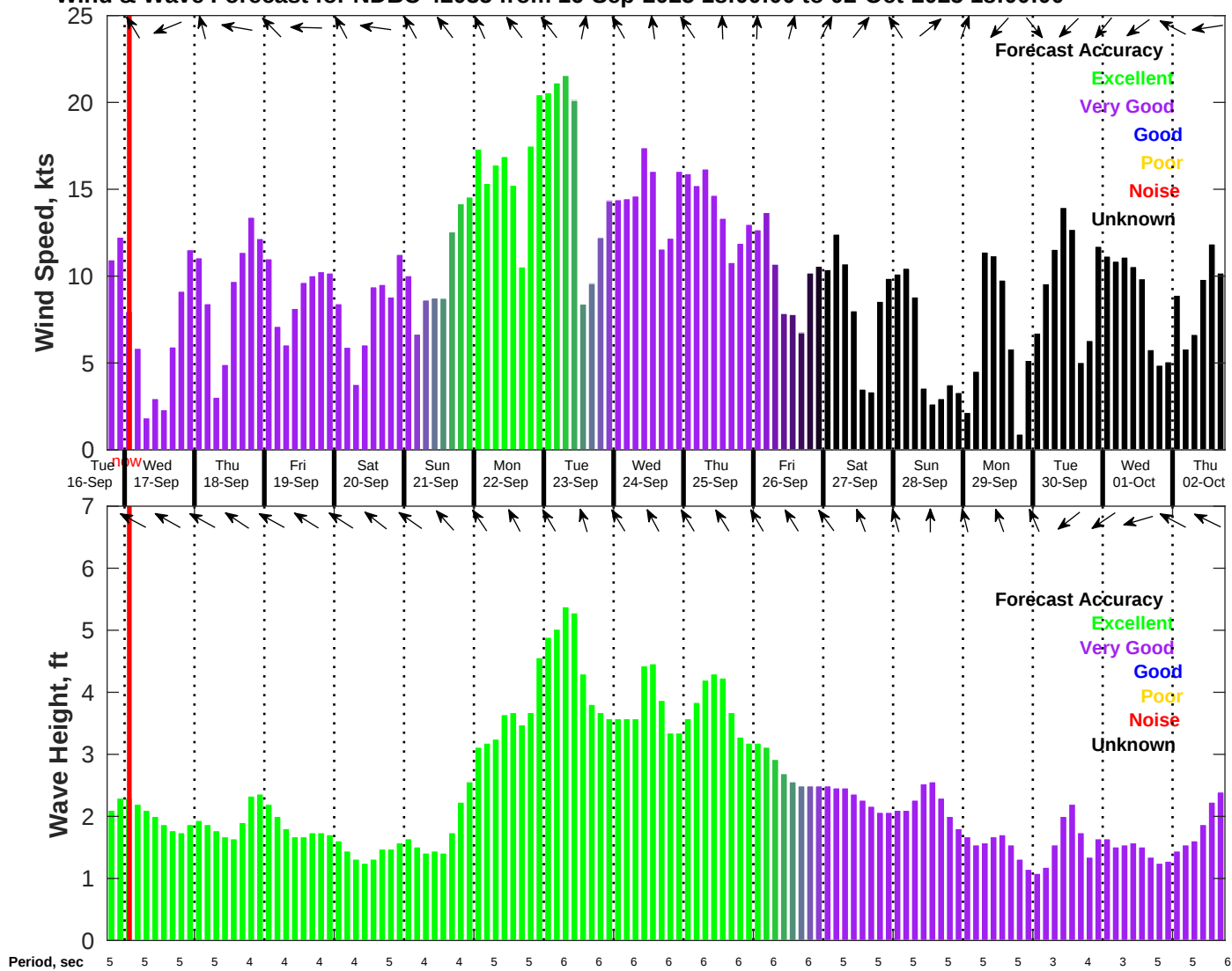
Wind & Wave Forecast for NDBC 42035 from 16-Sep-2025 18:00:00 to 02-Oct-2025 18:00:00
