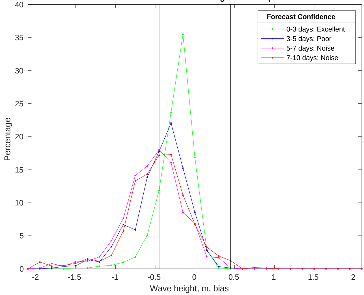
NDBC 42036 vs CMEMS Waves Bias Histogram: 17-Sep-2025
