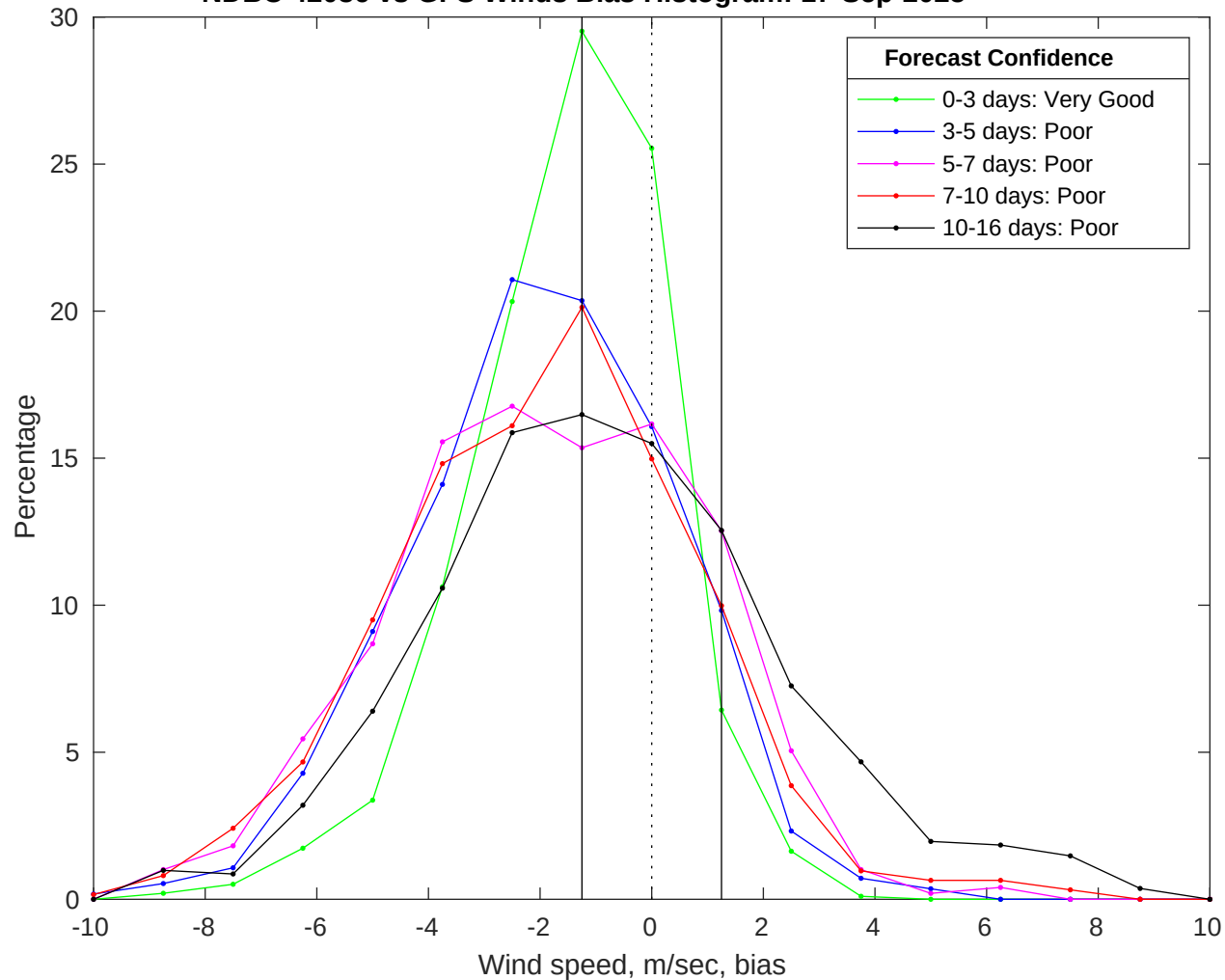
NDBC 42036 vs GFS Winds Bias Histogram: 17-Sep-2025
