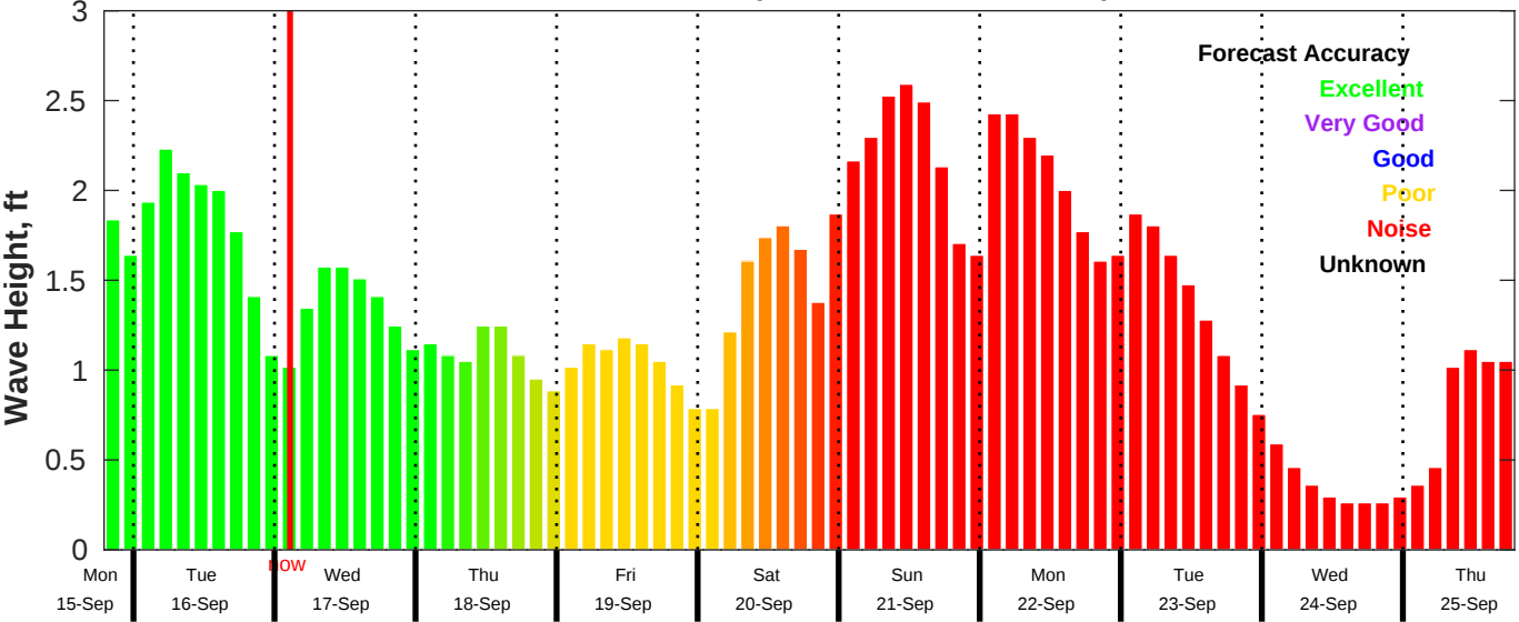
CMEMS Wave Forecast for NDBC 42036 from 15-Sep-2025 19:00:00 to 25-Sep-2025 19:00:00
