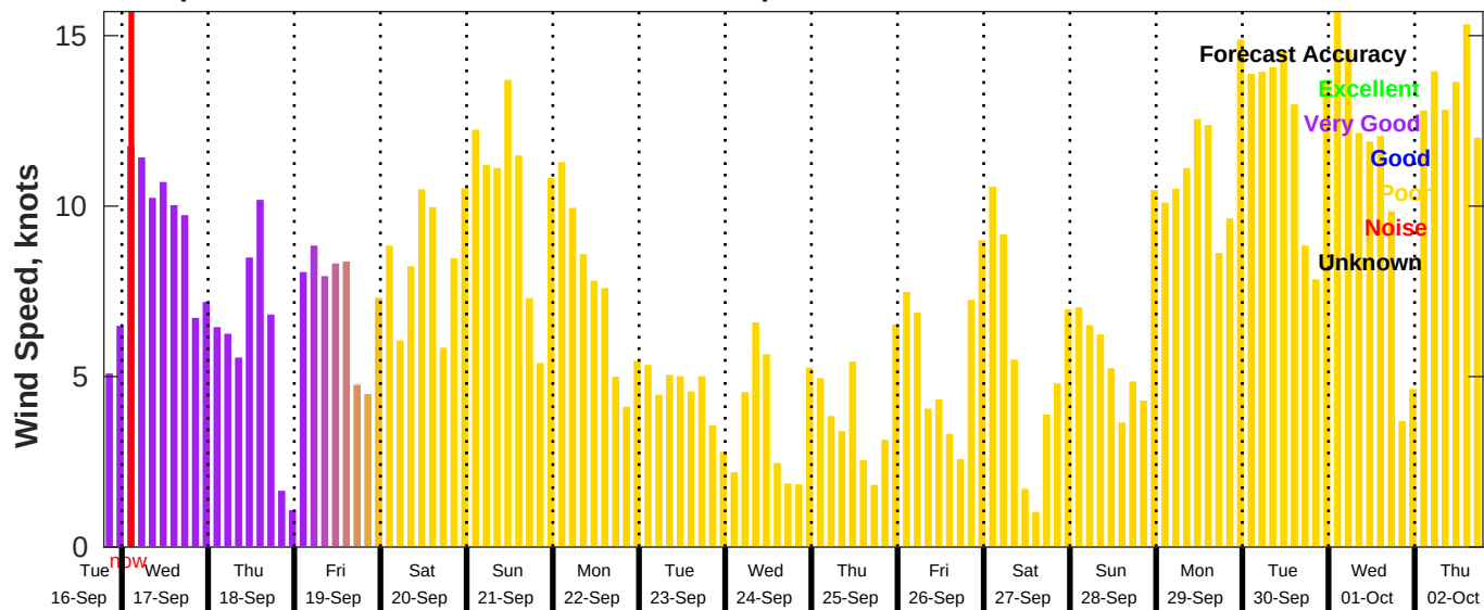
GFS Wind Speed Forecast for NDBC 42036 from 16-Sep-2025 19:00:00 to 02-Oct-2025 19:00:00
