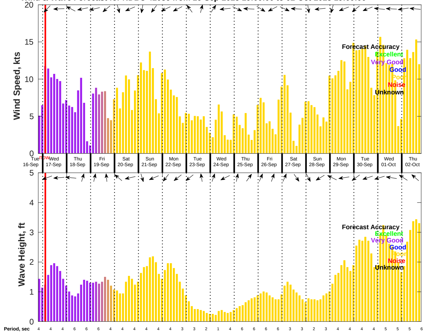
Wind & Wave Forecast for NDBC 42036 from 16-Sep-2025 19:00:00 to 02-Oct-2025 19:00:00
