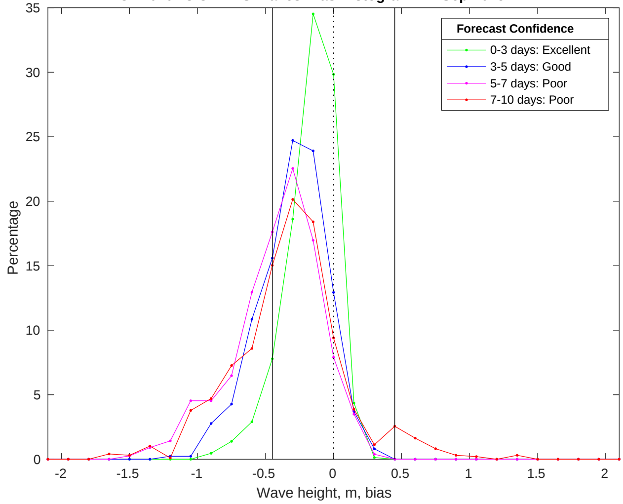
NDBC 42040 vs CMEMS Waves Bias Histogram: 17-Sep-2025
