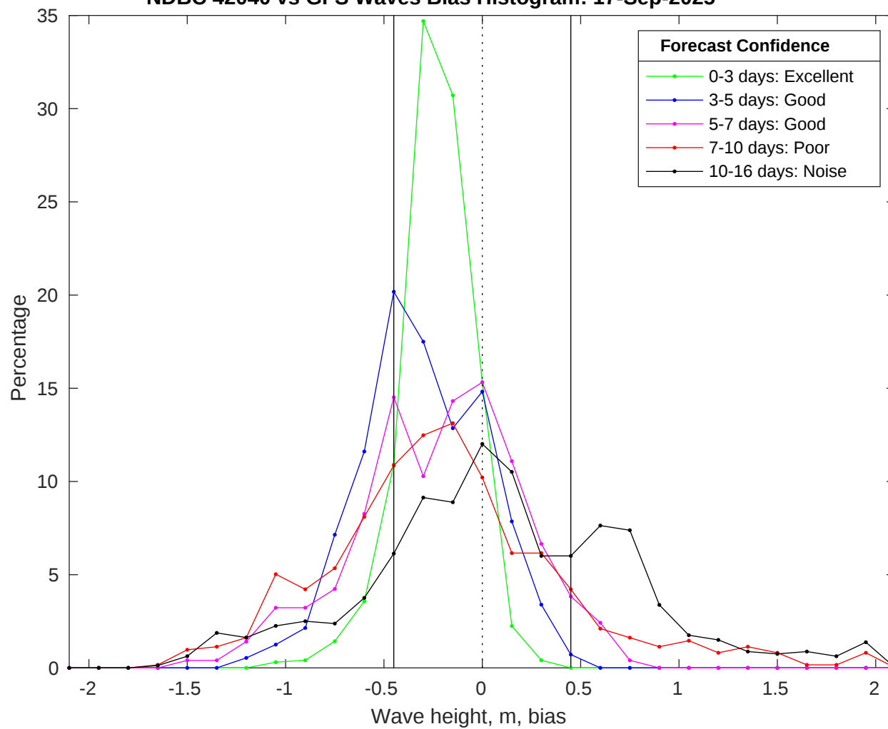
NDBC 42040 vs GFS Waves Bias Histogram: 17-Sep-2025
